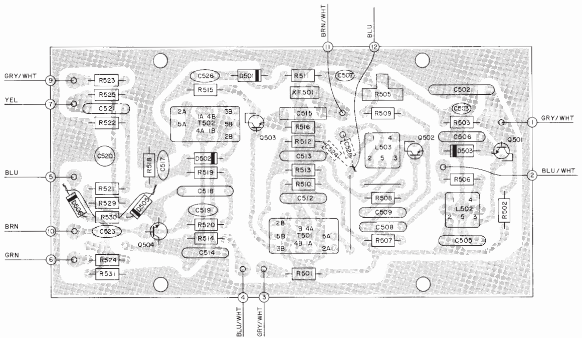
AM PC BOARD 044-276
