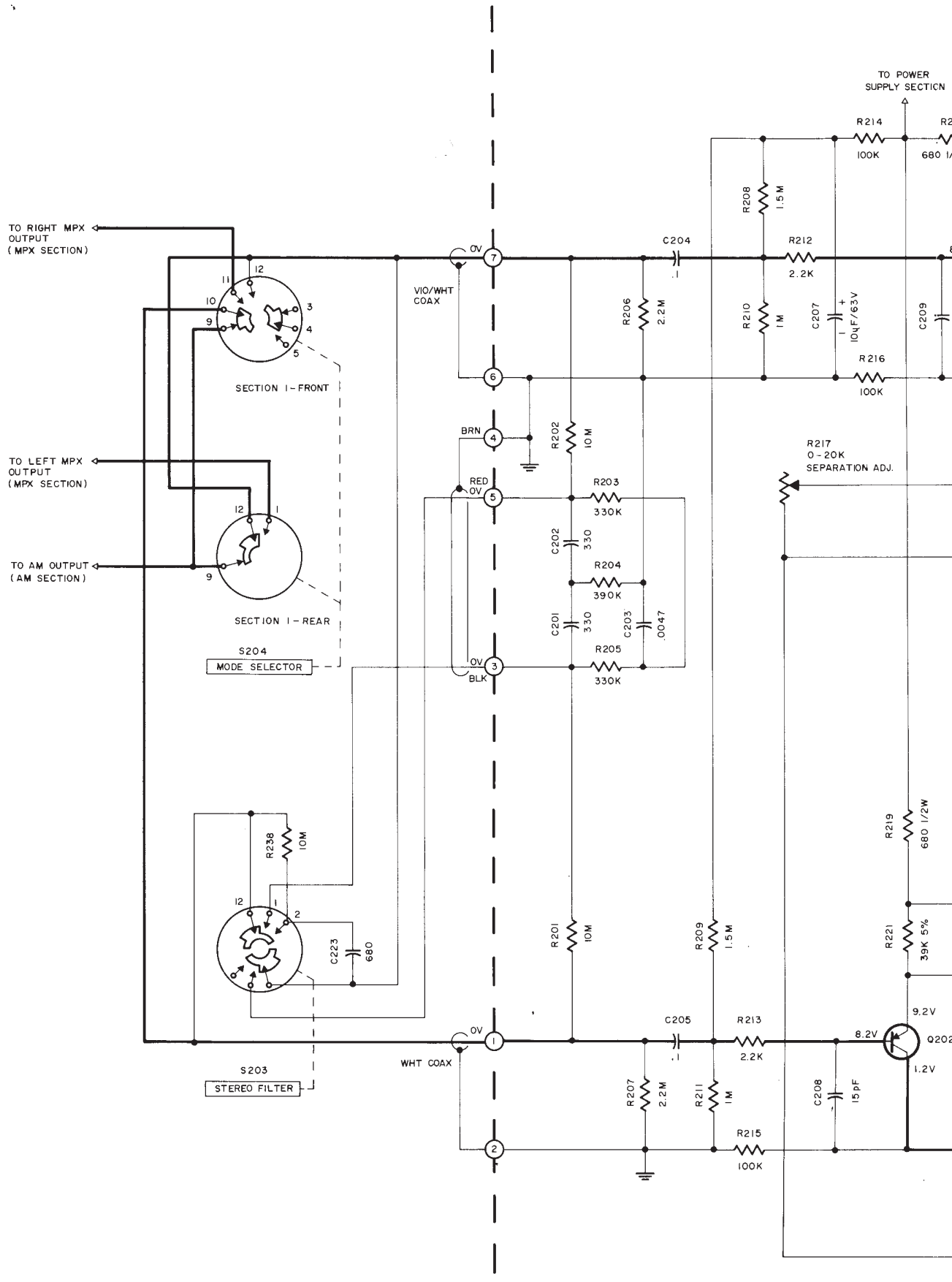
AMPLIFIER & VOLTAGE REGULATOR PC BOARD 044-
